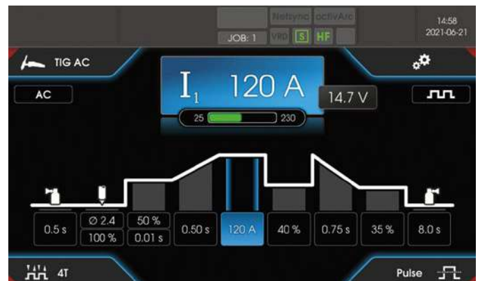
Graphic adjustment of all parameters in the flow diagram
